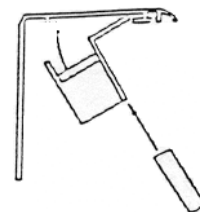
Glazing Block Detail
